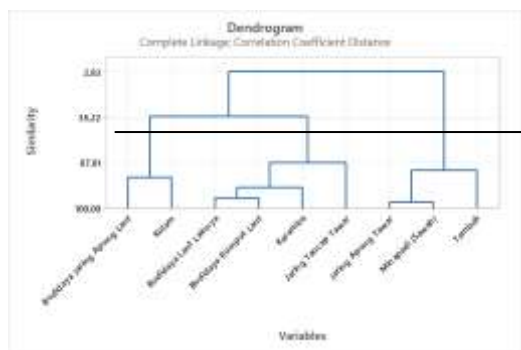
Image 3. Dendogram
