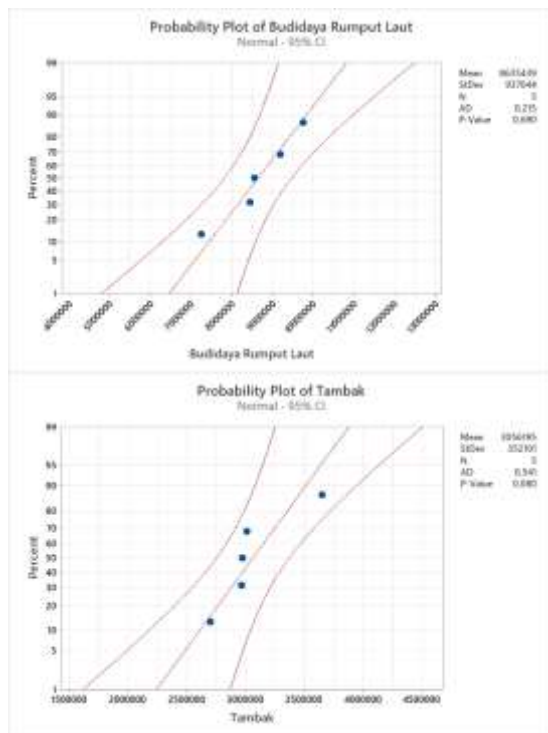
Image 2. Probability Plot
